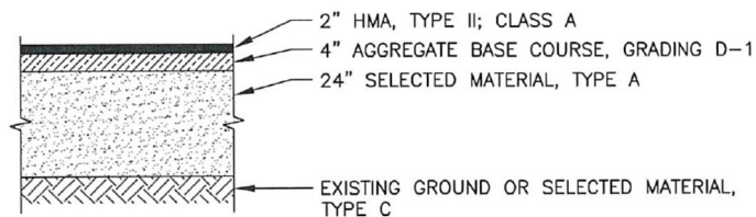
PAVEMENT STRUCTURAL SECTION NO.1
